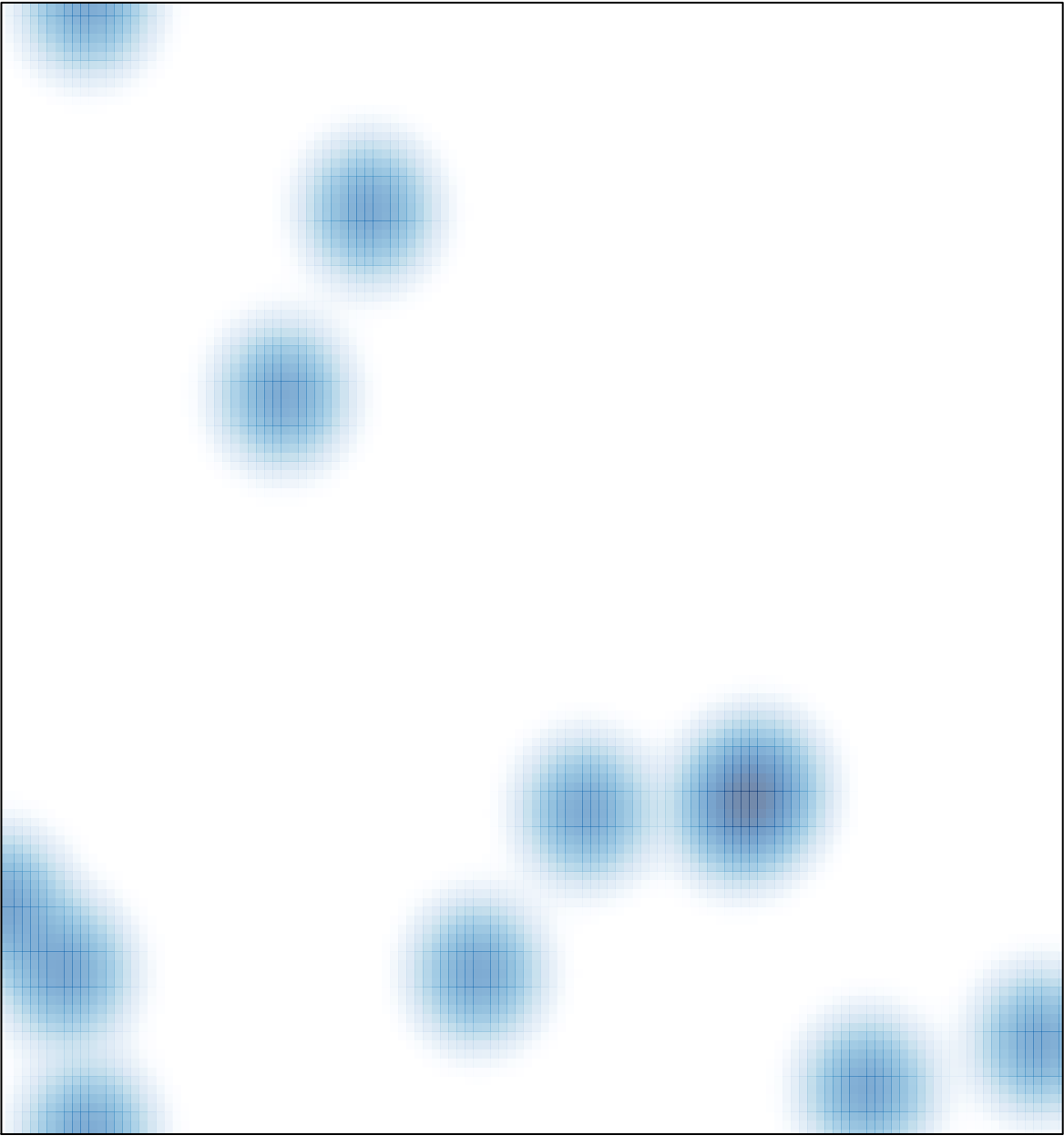
# features = 12 , max = 1
